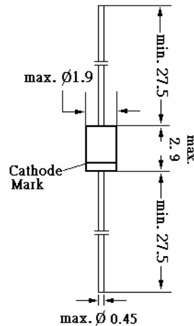
Glass case JEDEC DO-34 Dimensions in mm Weight approx. 0.092g
