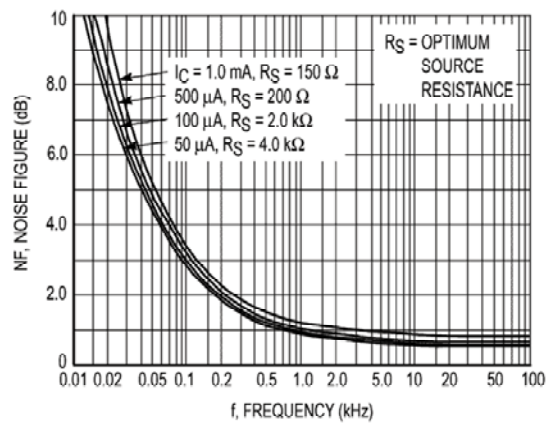
Figure 7. Frequency Effects
